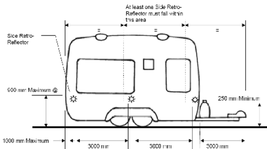
FIGURE 4 Side Retro-Reflectors – Dimensional Limits
