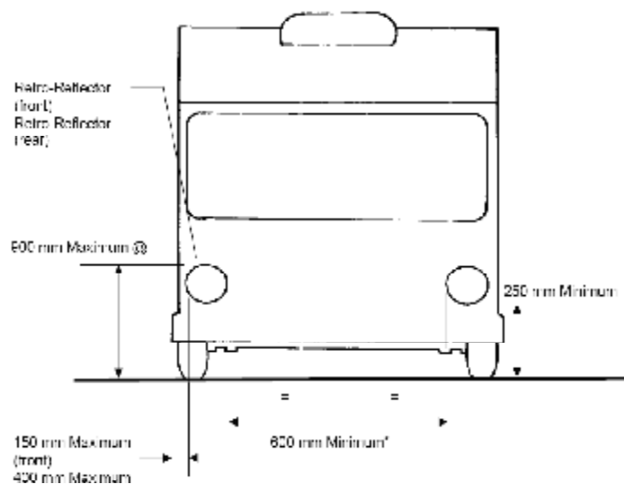
FIGURE 3 Front and Rear Retro-Reflectors – Dimensional Limits
